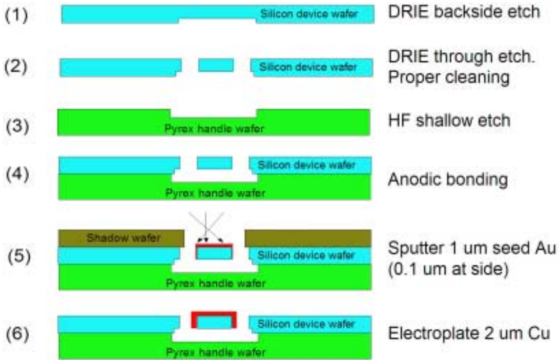
Figure 5-1 Key fabrication steps
