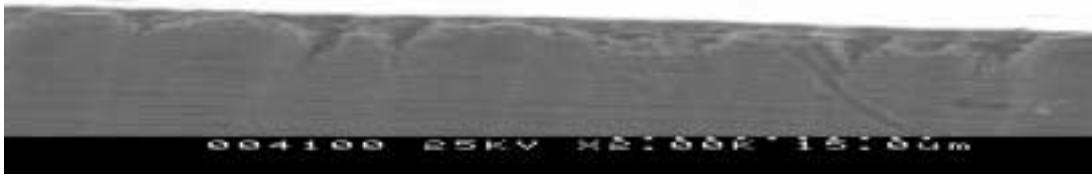
Figure 4-12 Poor metal continuity across the edge between wafer top and sidewall
