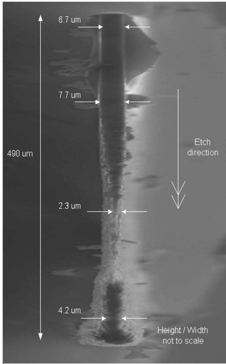
Figure 2-9 SEM of a beam fabricated with DRIE
