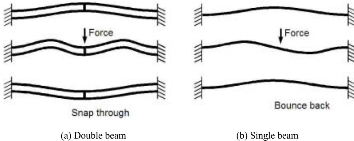
Figure 2-7 Double curved beam versus single curved beam
