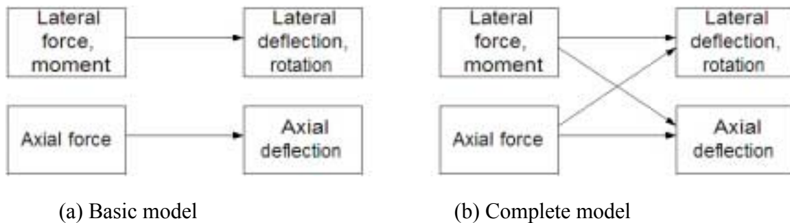
Figure 3-3 Treatment of the cantilever in the basic and the complete models
